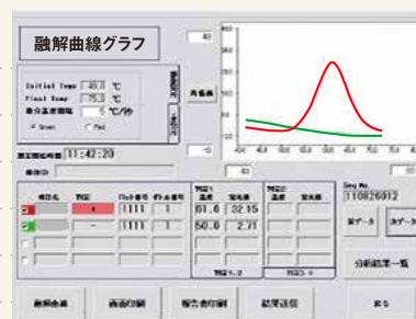
Reaction mixtures 1 2 3 4 5 6 7 8 9 10 100 P 50 P 30 P 20 P 10 P 5 P 3 P 2 P 1 P 100 80 60 40 30 20 10 5
